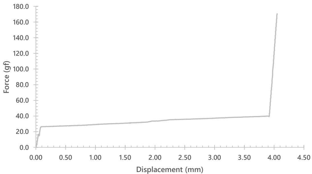
Keygeek Full Nylon (Upstroke)
